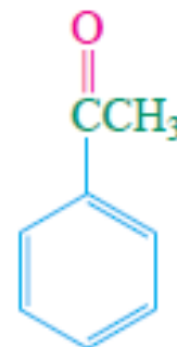
1-feniletanon (acetofenon)
