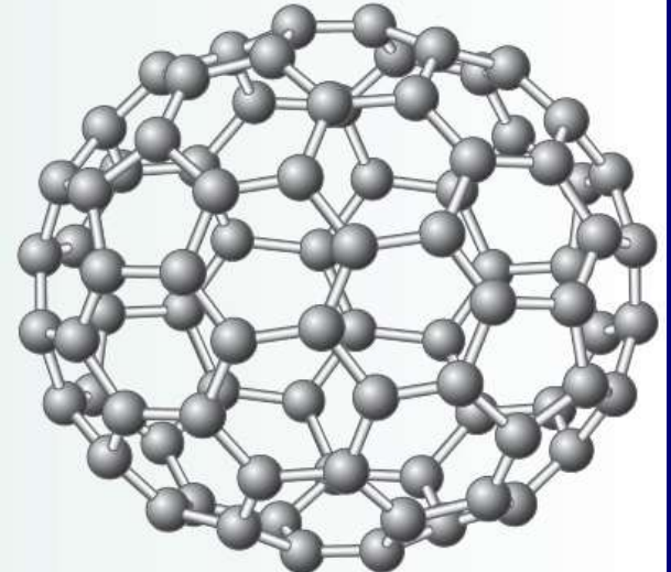
Chiral C 84
