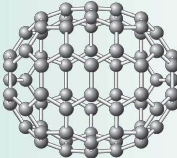
C 70
