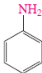
benzenamin (anilin)
