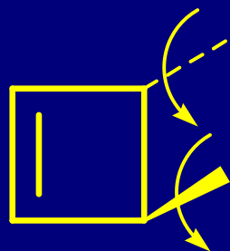
Trans
