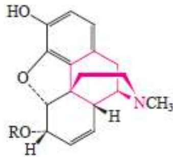
morfin (R = H) heroin (R = CH 2 C=O)
