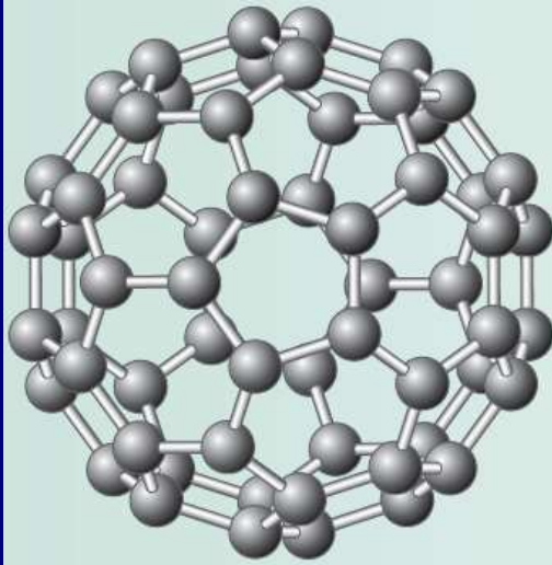
Buckminsterfullerene C 60
