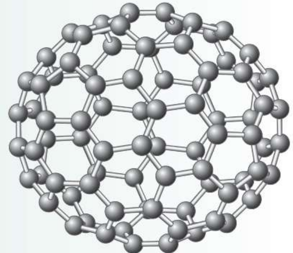
Chiral C 84
